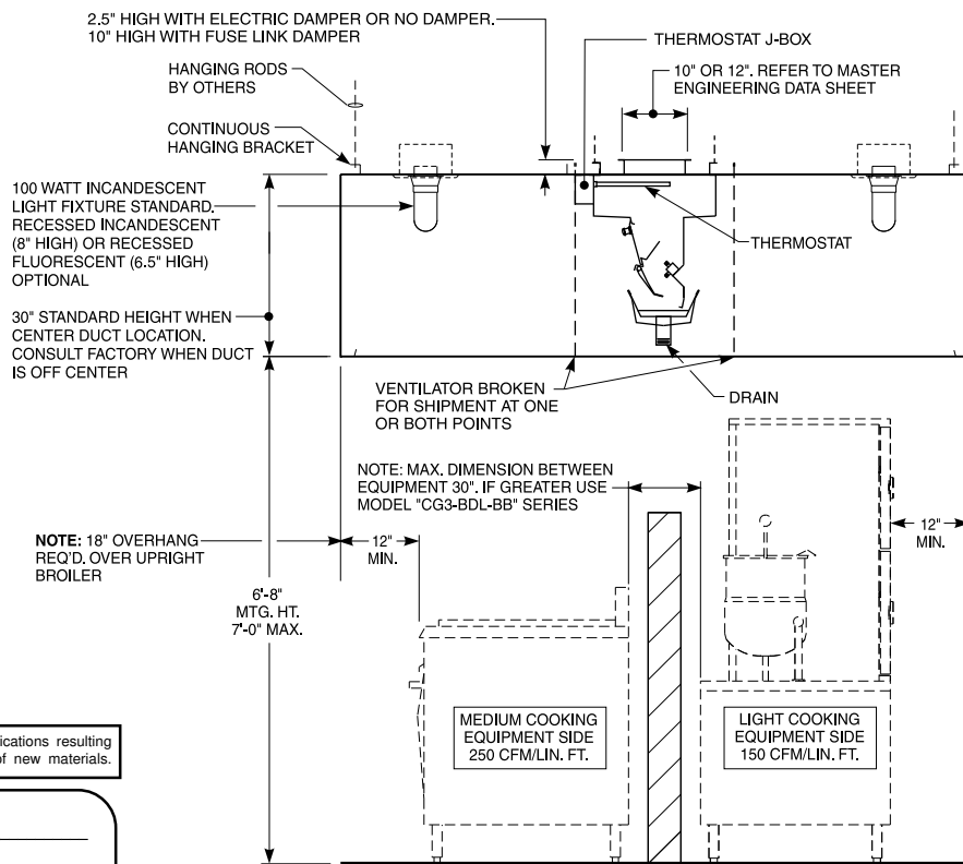
TYPICAL SECTION VIEW
